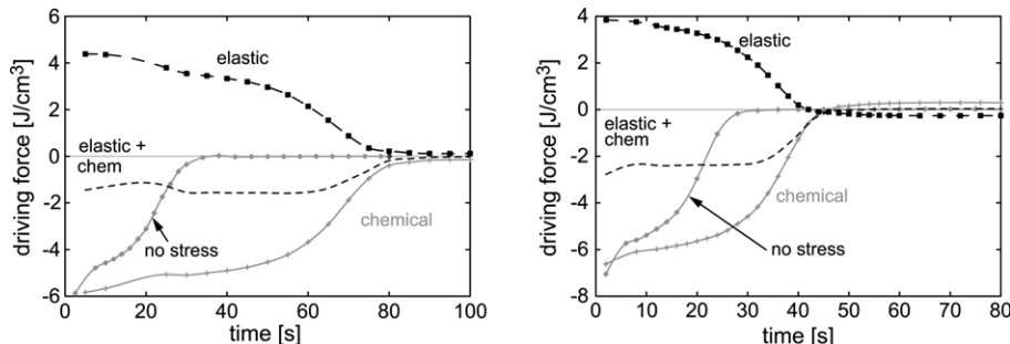
Fig. 5. Local driving force contributions at the interface as a function of time. Left: transformation at 1090 K. Right: transformation at 1085 K.
