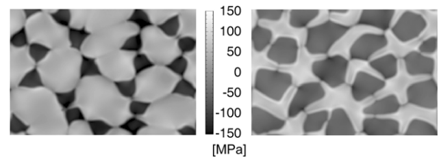
Fig. 8. Hydrostatic stress distribution within the structures of Fig. 7. Stress levels are in between -150 MPa and 150 MPa.
